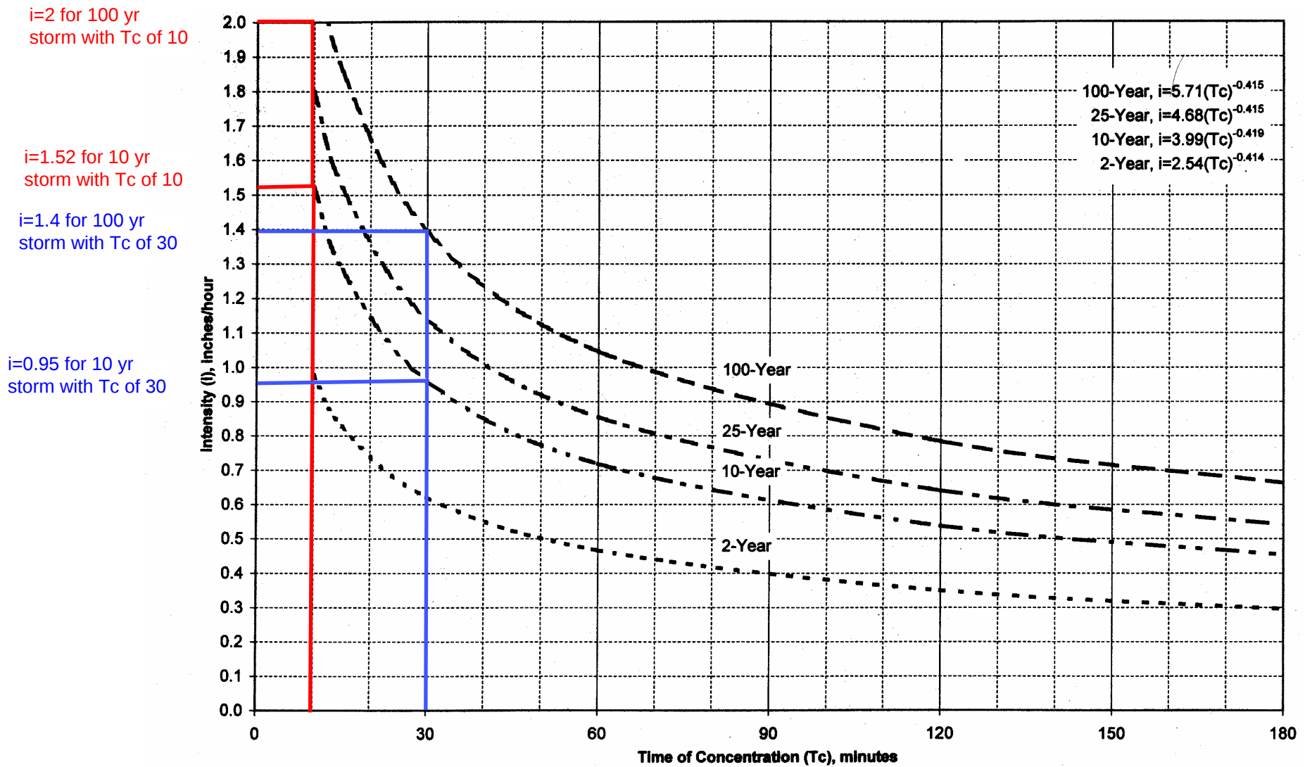
Figure 1: Rainfall Duration-Intensity Curves
