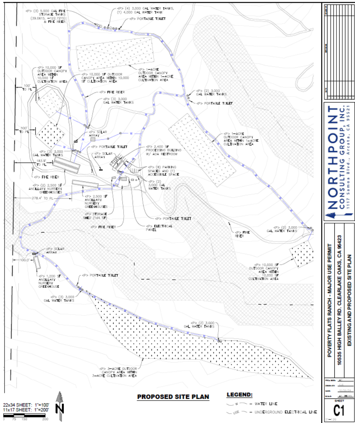
FIGURE 1 – SITE PLANS
