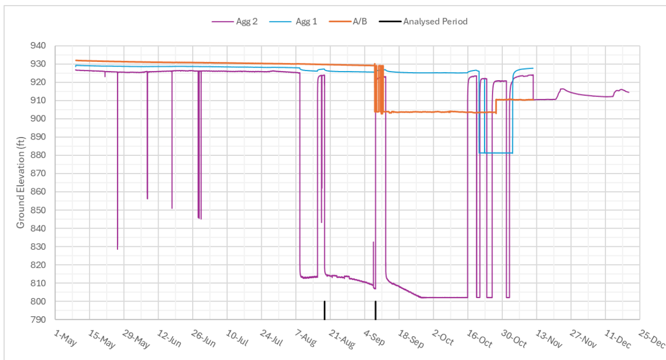
Figure 4 Transducer Data
