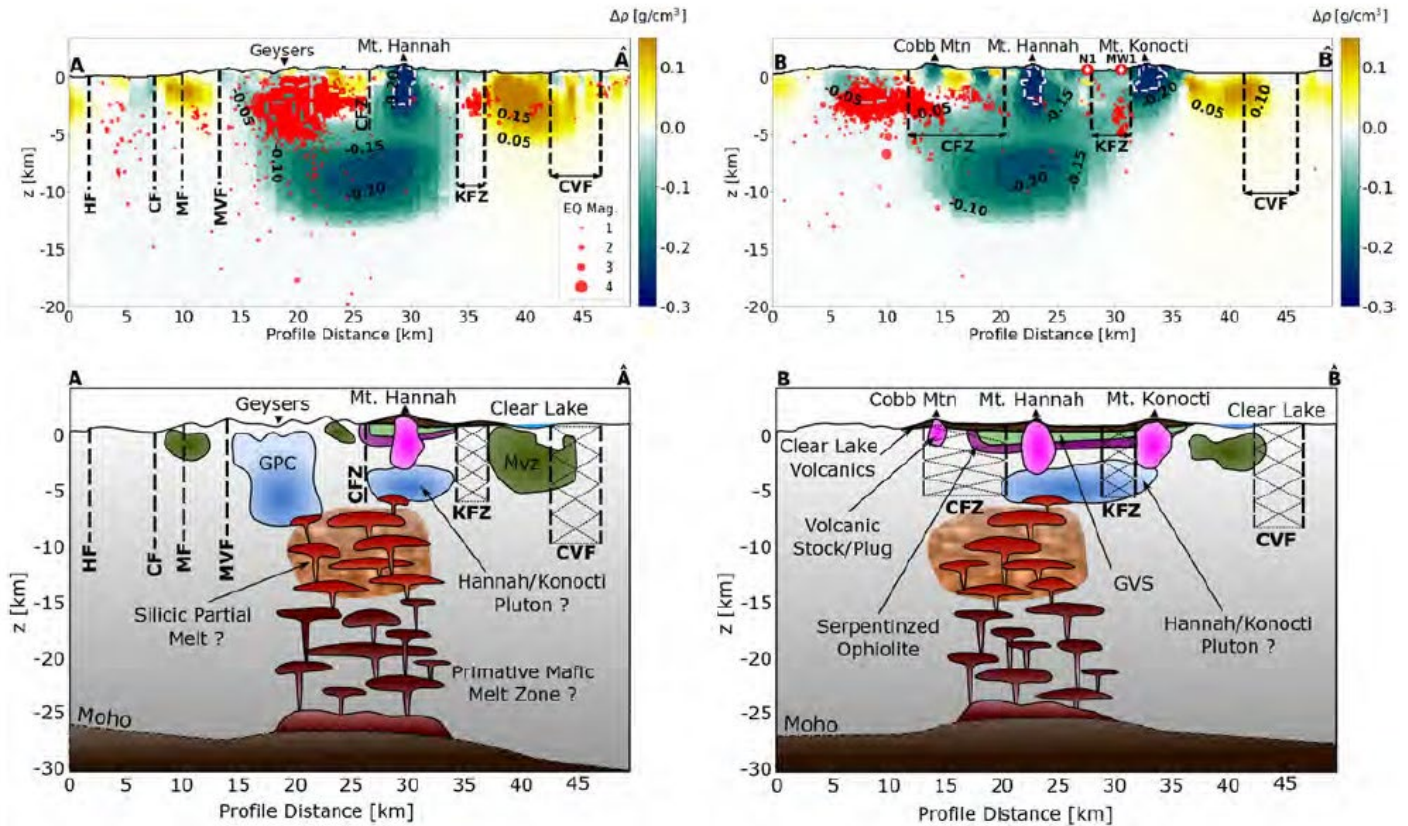
Fig. 23. Interpretive cartoons (bottom row) compared to A-A' and B-B' sections from the geologically constrained 5-unit PGI of the field dataset overlaid with the location of faults (vertical black dashed lines) and earthquake hypocenters (red dots) that fall within 1 km on either side of the profile (top row). The cartoons illustrate our interpretation of the subsurface geology based on the inversion results and the findings of previous studies. As in Fig. 1 faults are labeled in the following manner: HF-Healsburg Fault, MF-Maacama Fault, CF-Chianti Fault, MVF-Mercuryville Fault, CFZ-Collayomi Fault Zone, KFZ-Konocti Bay Fault Zone, and CVP-Clover Valley Fault. In the interpretive cartoons, Franciscan Complex rocks are gray, upper mantle rocks are black, the Geysers Plutonic Complex (GPC) is light blue, the Great Valley Sequence (GVS) is pale green, serpentinized ophiolites are purple, Mesozoic volcanics and metavolcanics (MVZ) are dark green, volcanic stocks/plugs are magenta and Clear Lake Volcanics are dark brown. The light brown, textured body overlaid with reddish orange sills between 6 and 13 km depth shows the proposed silicic partial melt zone, and the dark red sills show the inferred primitive mafic melt zone beneath it.
