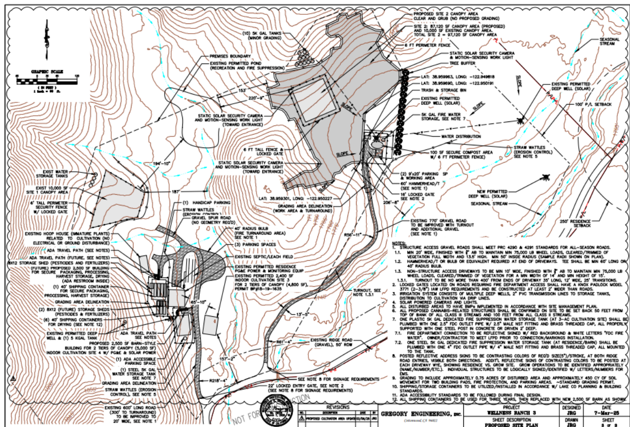
FIGURE 1 –SITE PLAN
