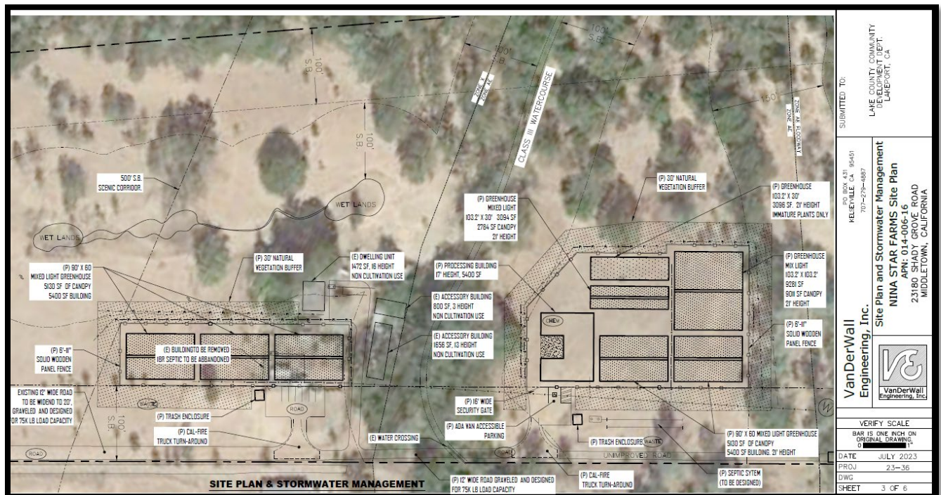
FIGURE 2 – SITE PLANS
