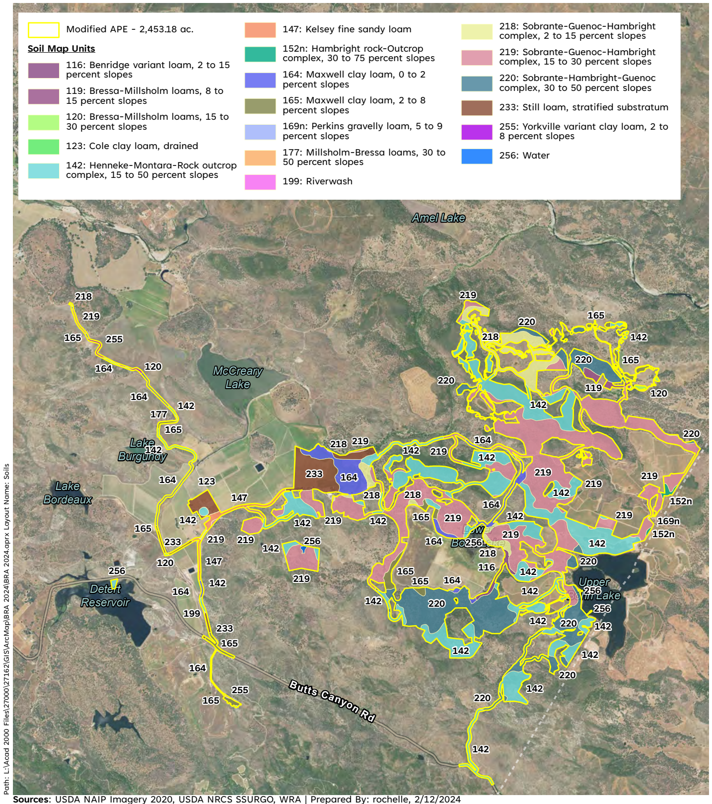
Figure 3. Soil Types within the Modified APE
