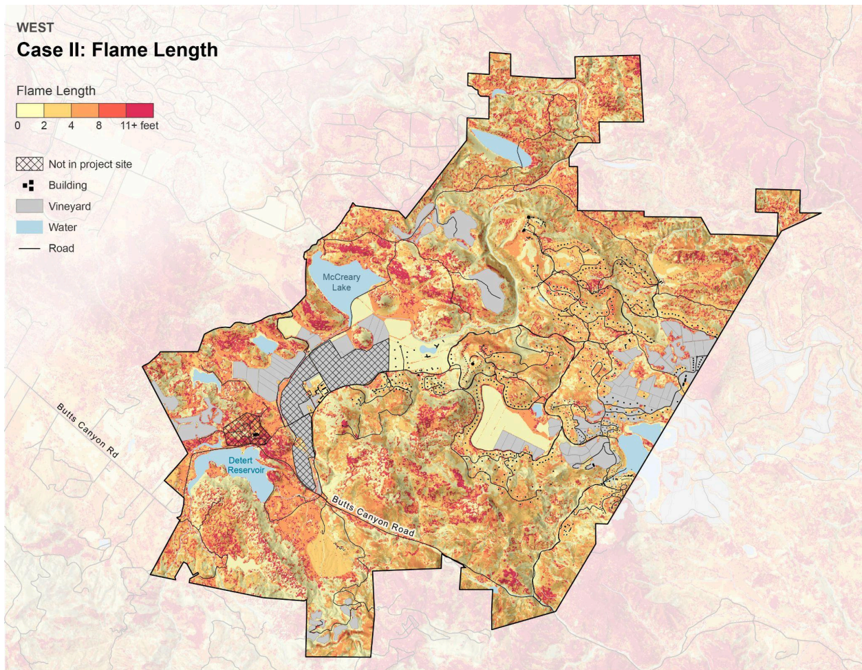
Figure 5.9: projected flame length under Case II
