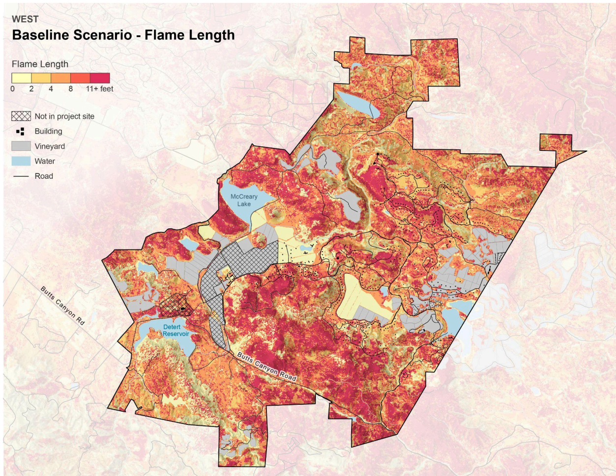
Figure 5.6: Modeled flame length under the existing baseline conditions
