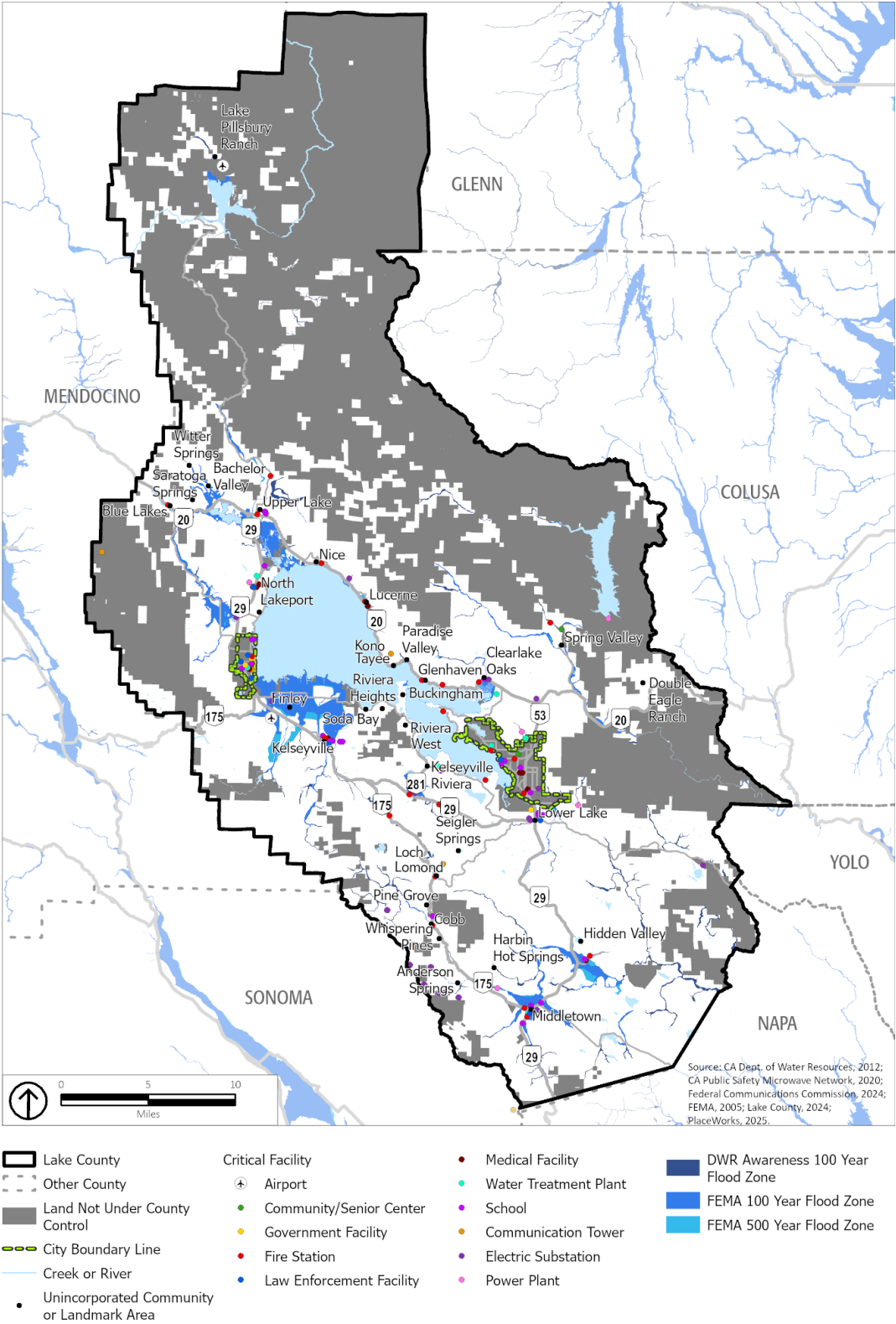
Figure C-6 Flood Hazard Zones in Lake County
